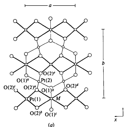
Fig. 3. (a) ORTEP drawing of the C-centered MPt_3O_6 structure projected down [001].
